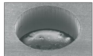
Drilling titanium
