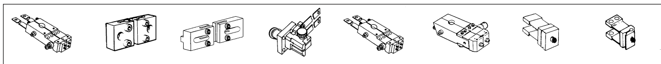
HE87 HOLDERS, UNITIP/THERMODE for 87F and 87A. HE88 ELECTRODE HOLDER Holder .245 in dia. ES0800 Series electrodes in 88 Weld Head. Set (2) HE188 ELECTRODE HOLDER Holder .245 in dia. ES0800E Series electrodes in 188 Weld Head. Set (2) HE50 HOLDERS, UNITIP for 50F and 50A Weld Heads. HE50RF HOLDER, THERMODE , for 50F and 50A Weld Heads. HE50UB FLEXURE SET holds Unibond electrodes and Unitip adapter in 50 Weld Head. .HE127SFRE ROUND ELECTRODE HOLDER SET Holds 1/8 in dia. electrodes in 86 Weld Heads. Set (2) HE127SF STANDARD FIXTURE SET Holds Unibond electrodes in 86 Weld Head. Set (2)
