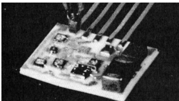
Thermocompression bonding gold leads to gold substrate pads is an easy task for the "T" tip thermode.
